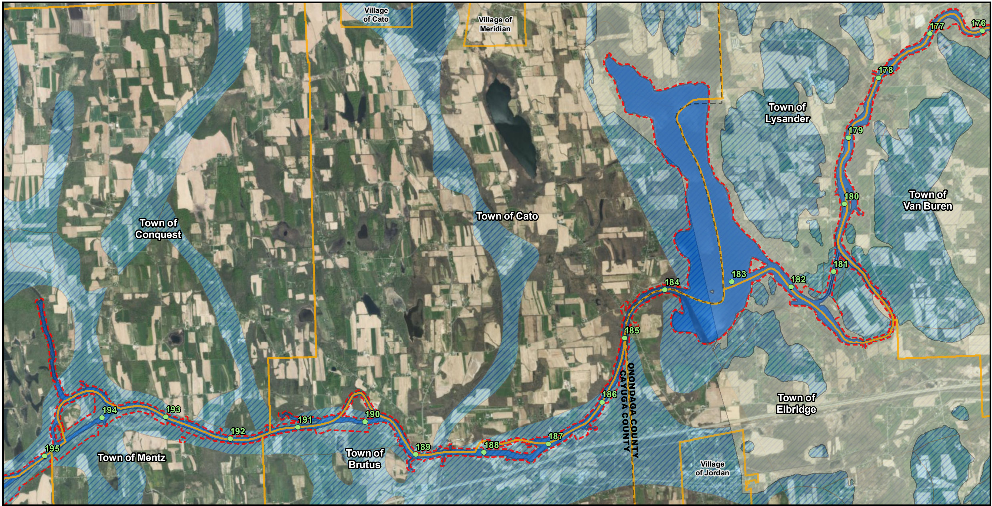
Figure 80F: Aquifers
